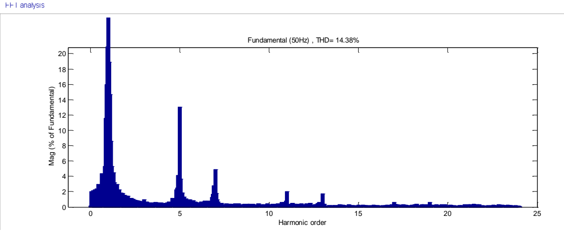
Fig 6.10 (b) : Source current (FFT) unless two inverters (THD =14.38%).
