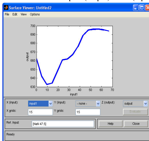
Figure 20: Anfis Speed versus load
