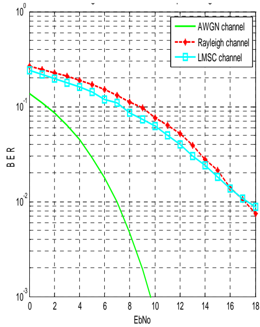
Figure 13. BER comparison of the Rayleigh and LMSC channels at 20 km/h
