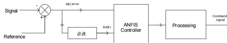
Figure 3: shunt APF control block diagram
