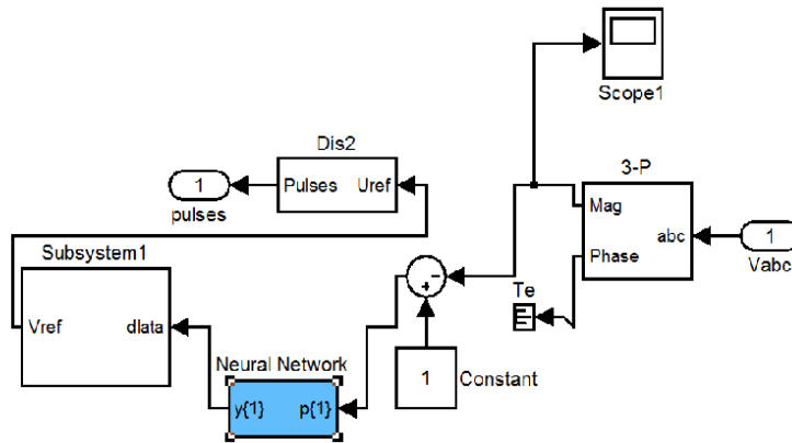
Figure 5. Voltage controller using neural networks
