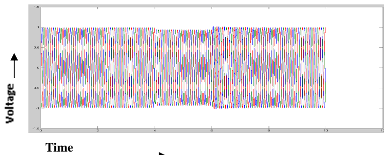
Figure 15. Load voltage with artificial neural network
