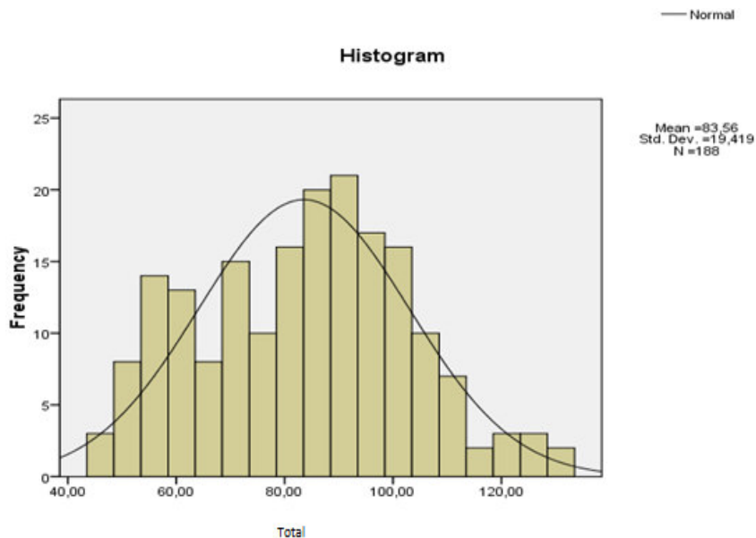
Figure 2. The Attitude Scale Frequency Graphics after the Extreme Values Were Excluded
