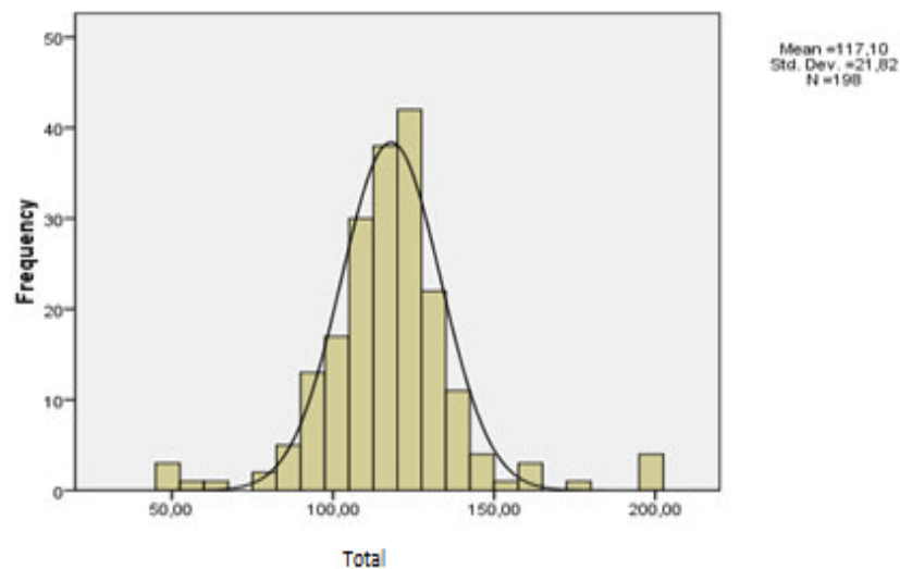
Figure 1. Attitude Scale Frequency Graphics
