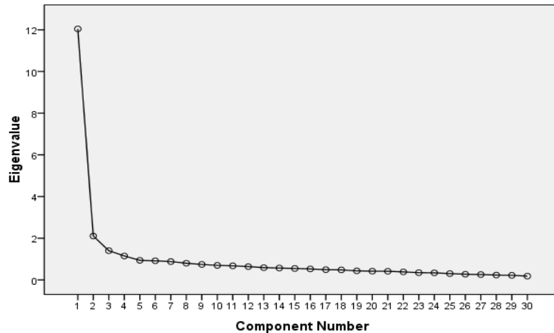
Figure 3. Scree Plot Graphics
