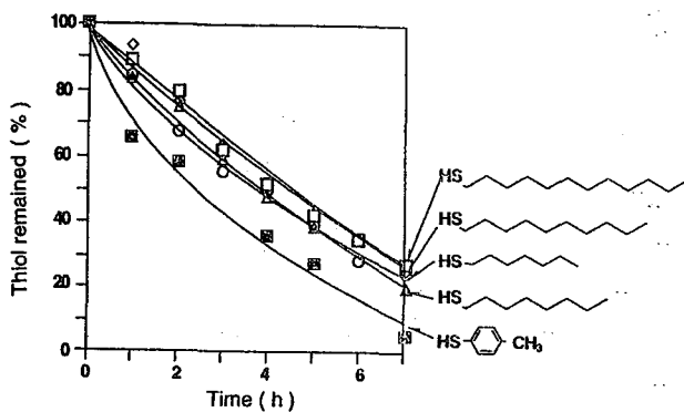
Figure 4. Sonochemical disappearance of thiols in i -ProOH / H 2 O (8:3)
