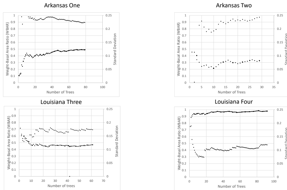
Figure 4. Running mean of the Weight-Basal Area Relationship (WBAR) of individual trees as additional “Full” points are measured. Weight is merchantable sawlog weight for Arkansas Two, Louisiana Three, and Louisiana Four but is merchantable pulpwood weight for Arkansas One since pulpwood is the most valuable product class on that site. For Arkansas One pulpwood is for both trees allocated only to pulpwood and those trees that have only upper-stem pulpwood (or topwood). The inclusion of upper-stem pulpwood adds substantial variability. Black circles are “running” means and black triangles are “running” standard deviations.
