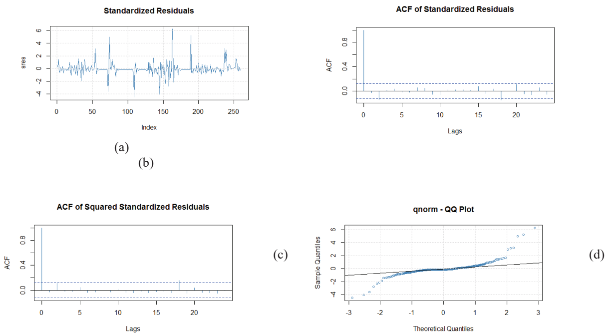
Figure. 8. Model diagnostics of the residuals from ARIMA(1,1,2)-ARCH(1) on log LRD/USD growth rate from Jan. 07, 2013 to Dec. 25, 2017: Parts (a), (b) (c) and (d) are the standardized residuals, ACF of standardized residuals, ACF of squared standardized residuals, and the Q-Q plots of the fitted model.
