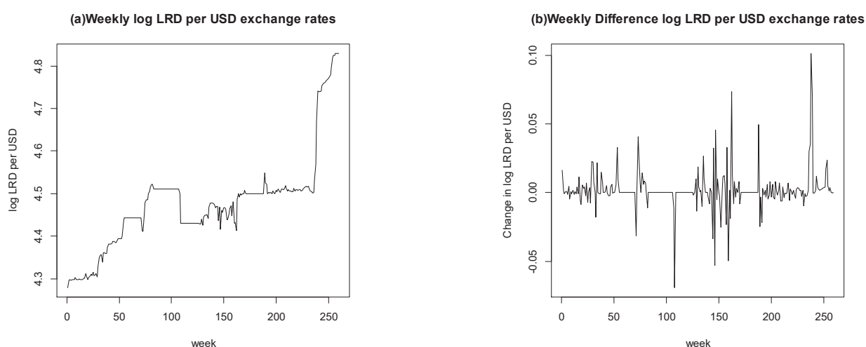
Figure 1: LBR/USD weekly exchange rate from January 7, 2013, to December 25, 2017. Weekly series of Liberia exchange rates in natural logarithms \{\ln x in (a), and the weekly growth rates \{\text{LRD-USD} = \Delta \ln x in (b).
