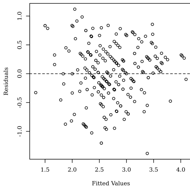
Figure 2 . Residuals scatter plot for homoscedasticity for TA, TB, TC, and TD predicting TE
