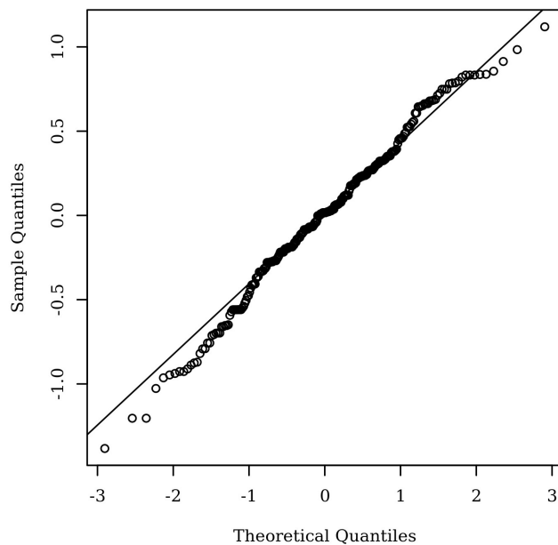
Figure 1. Q-Q scatter plot for normality for TA, TB, TC, and TD predicting TE
