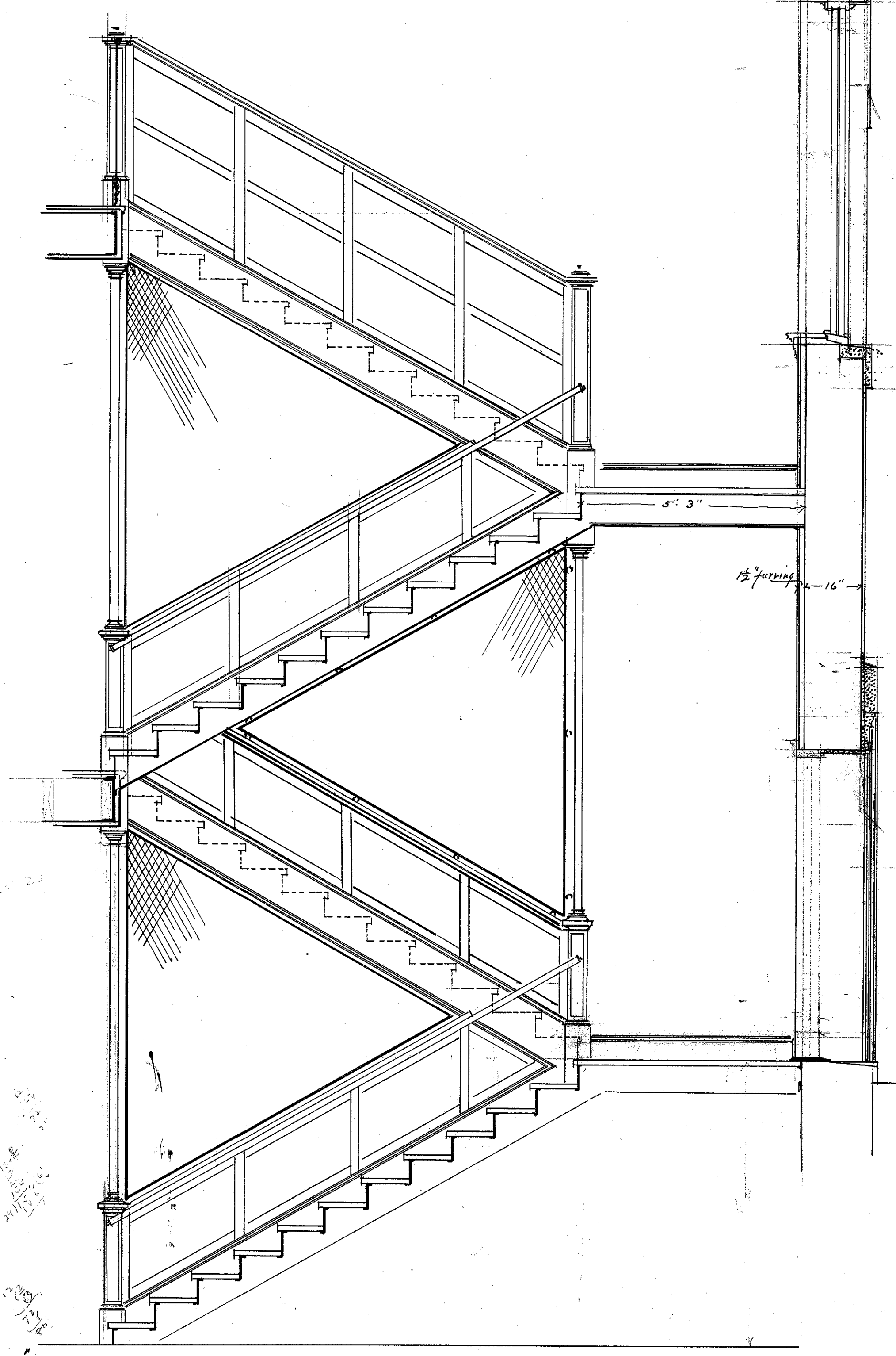
Section through East Stairs
