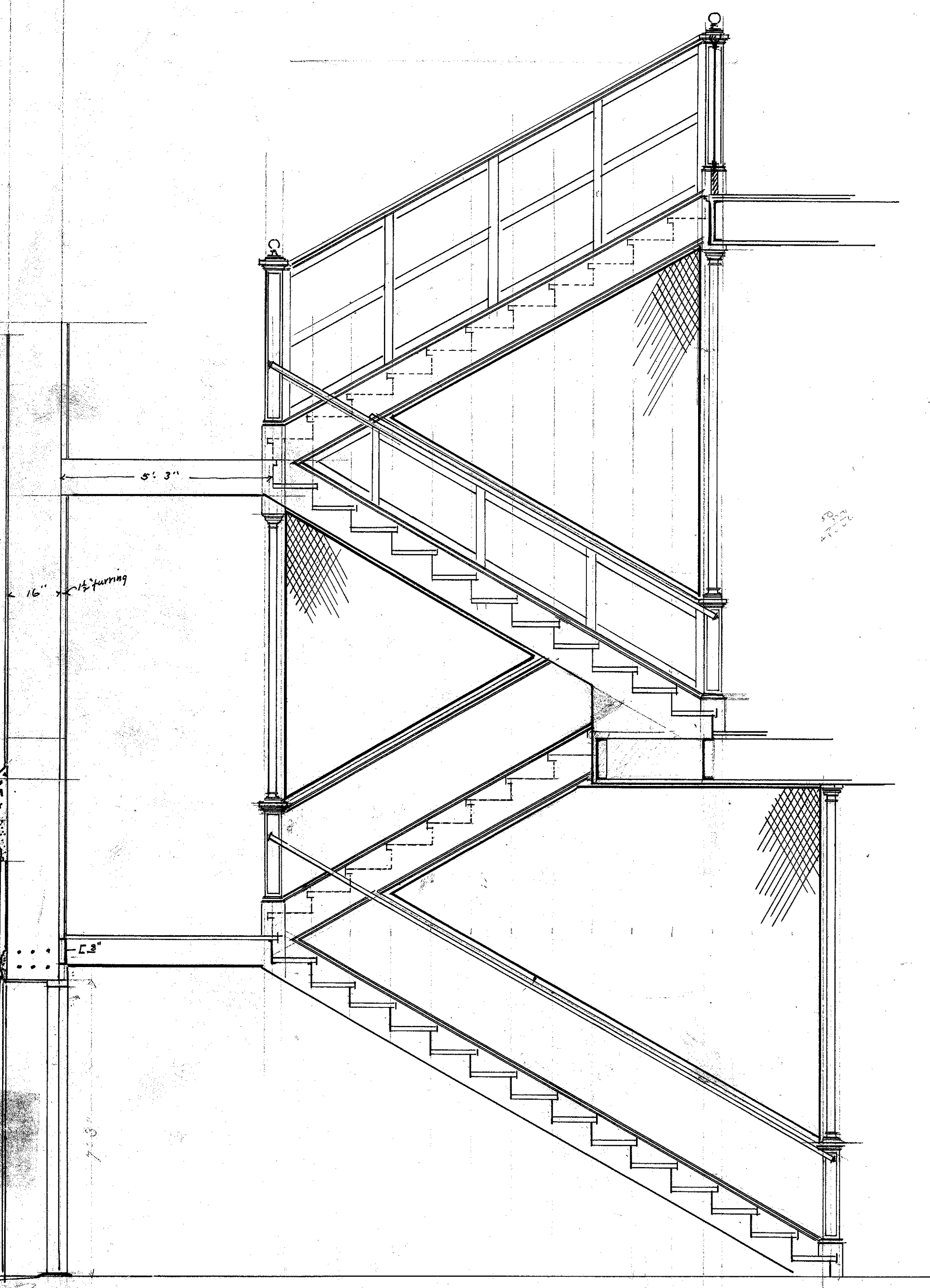
Section through West Stairs
