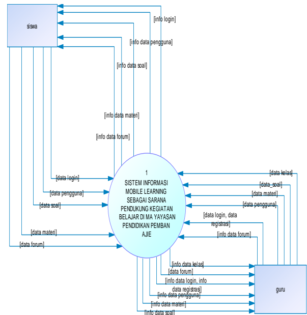
Gambar 1. Context Diagram
