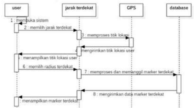
Gambar 8. Sequece Diagram Jarak Terdekat
