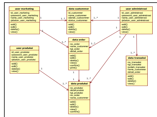
Gambar 4. Class Diagram
