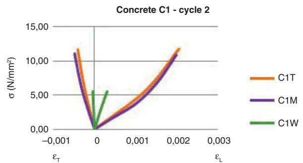
FIGURE 5. Second loading cycle. Results for C1.
