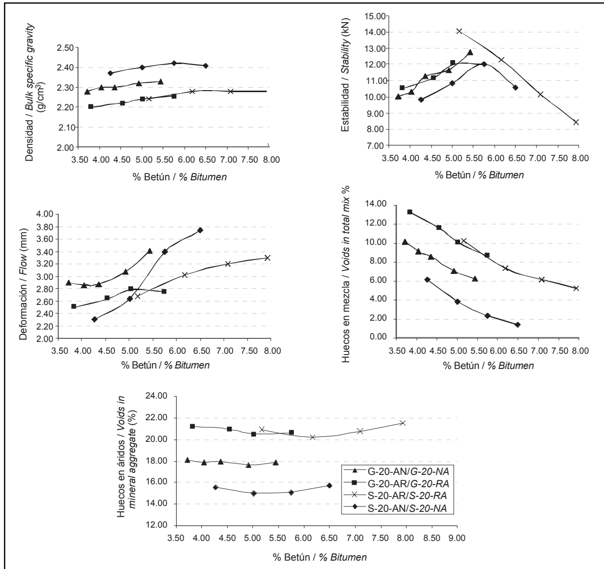
Figura 1. Ensayo Marshall. Figure 1. Marshall Test.
