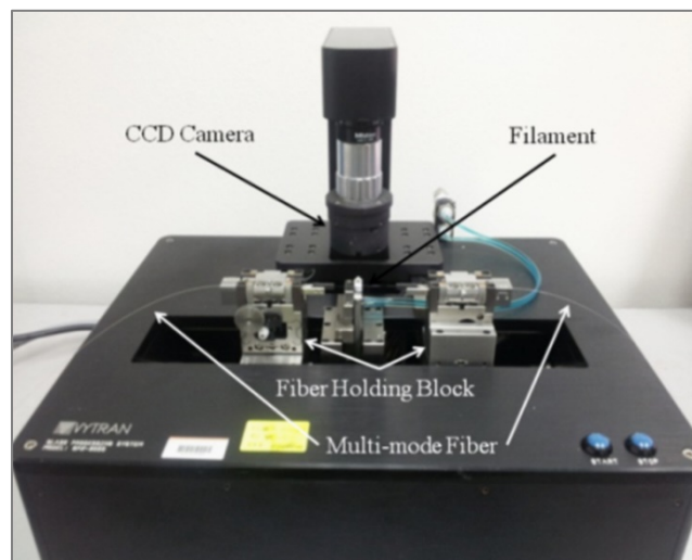
Figure 2: Optical Fiber Tapering Equipment (Vytran) (Shabaneh, et al., 2014)
