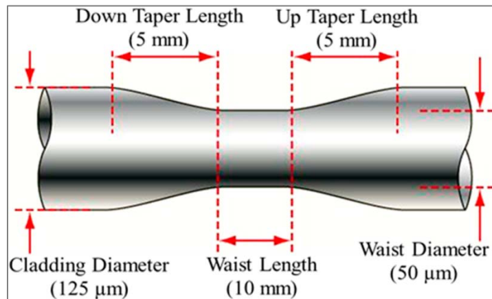
Figure 1: Tapered optical fiber parameters (Shabaneh, et al., 2014)
