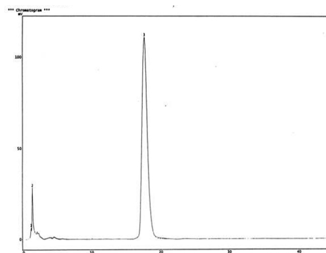
Figure.2. Chromatogram of Anacardic acid.
