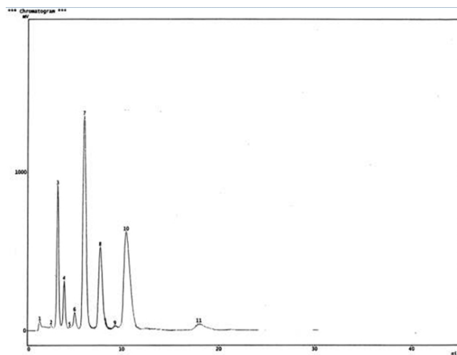
Figure.1. Chromatogram of CNSL.
