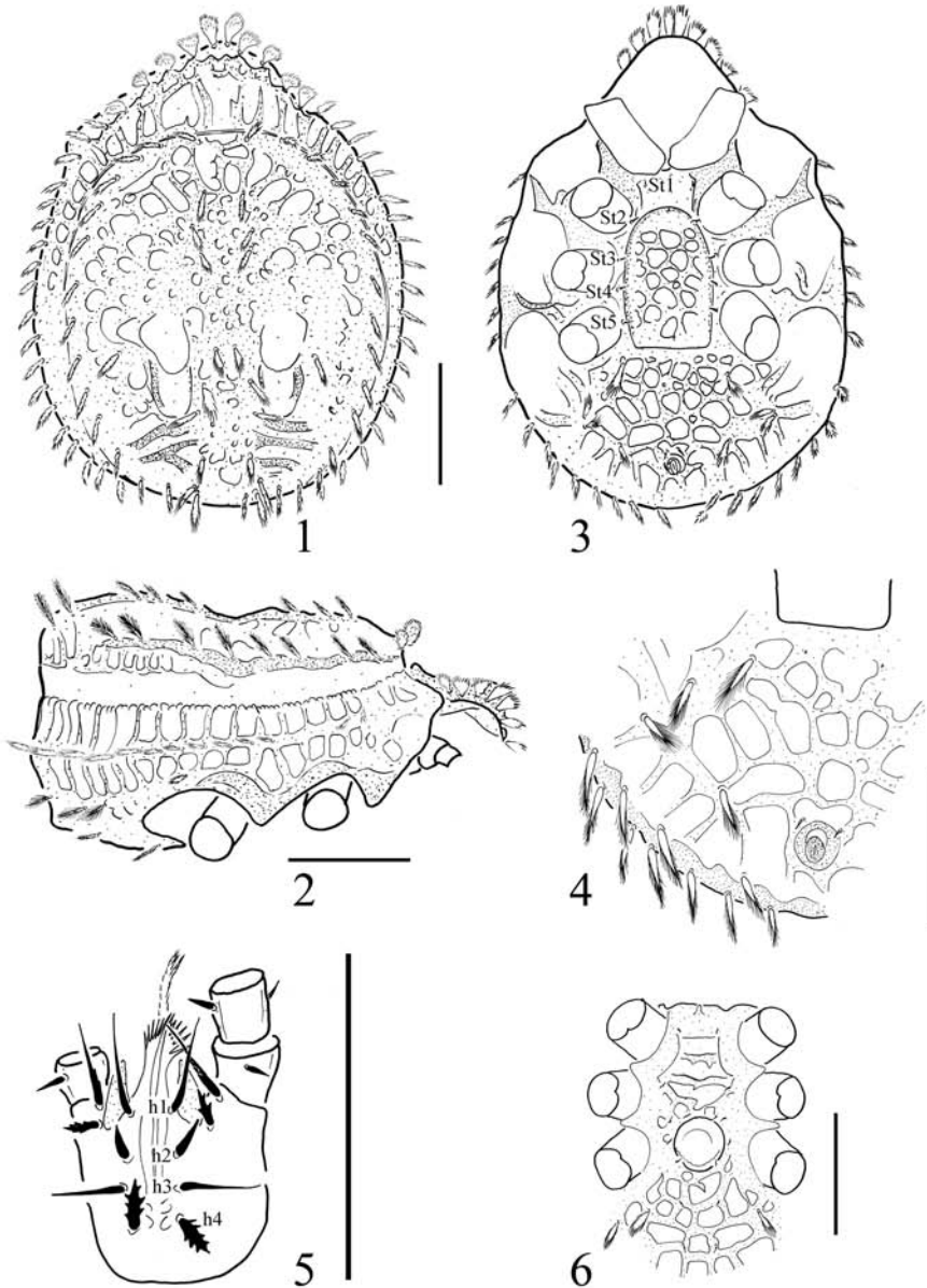
Figures 1-6. Uroobovella vazquezae sp. nov. 1: dorsal view, 2: lateral view, 3: ventral view, 4: ventral cavities and setae, 5: ventral view of gnathosma (female, holotype), 6: sternal region (male, paratype) (Scale bars: 100 \mu m).
