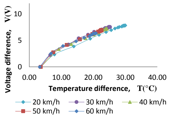
Figure 8. Changes in voltage difference ( V ) to the temperature difference ( T ), with a 175 V voltage regulator
