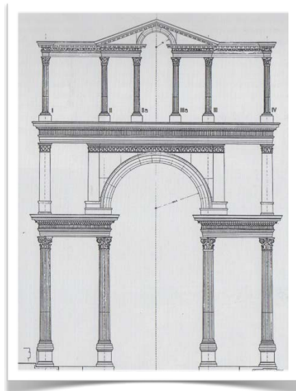
Figure 77. Reconstruction of Hadrian's Gate.
