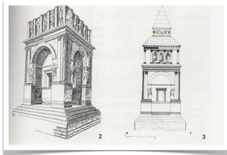
Figure 28. Reconstructive evolution of the Memmius Monument. The left hand side drawing was the initial suggestion, but this has since been modified to the structure on its right.
