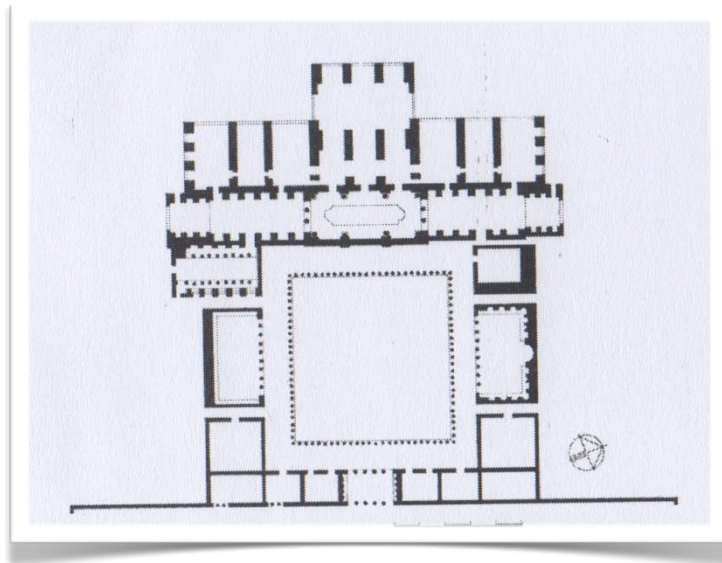
Figure 108. Floor plan of the Harbour Baths and Gym.
