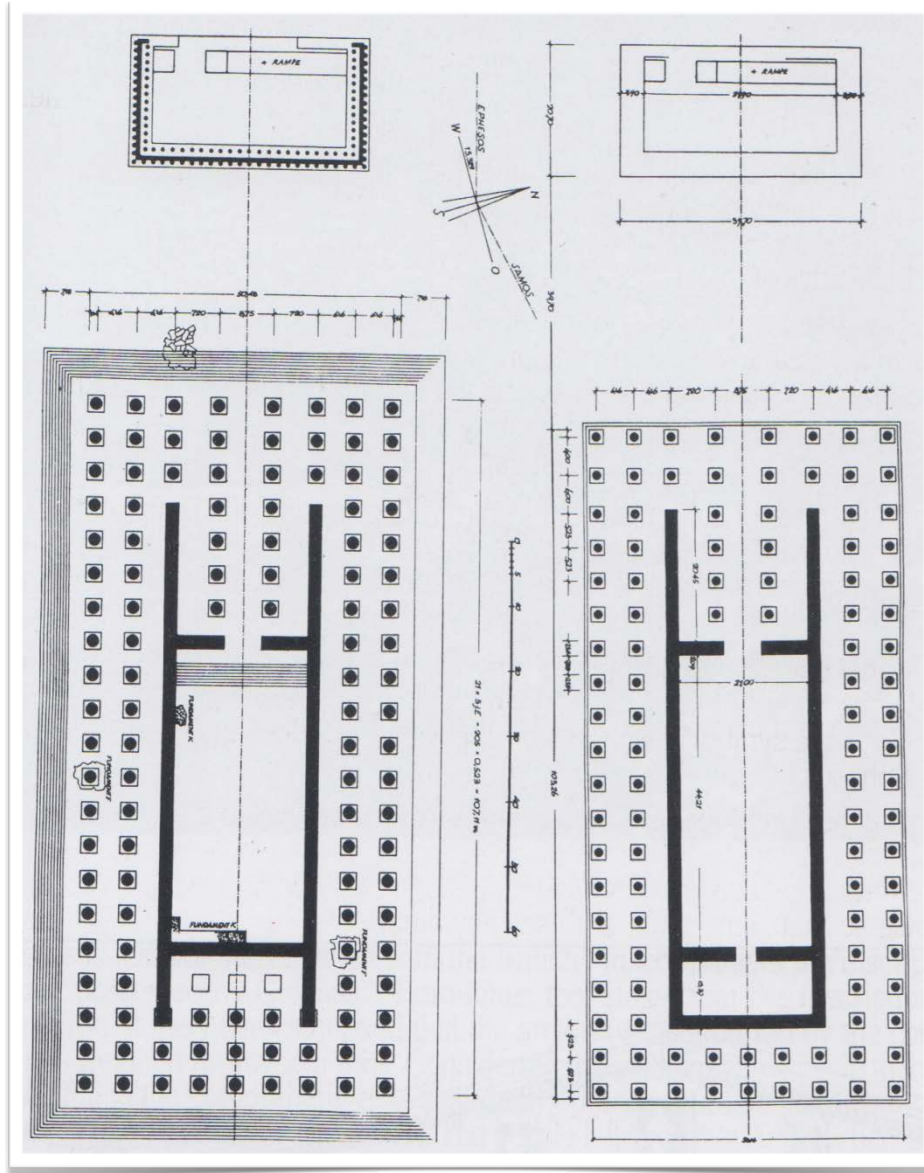
Figure 129. The Hellenistic temple floor plans on the left and the Archaic temple floor plans on the right.
