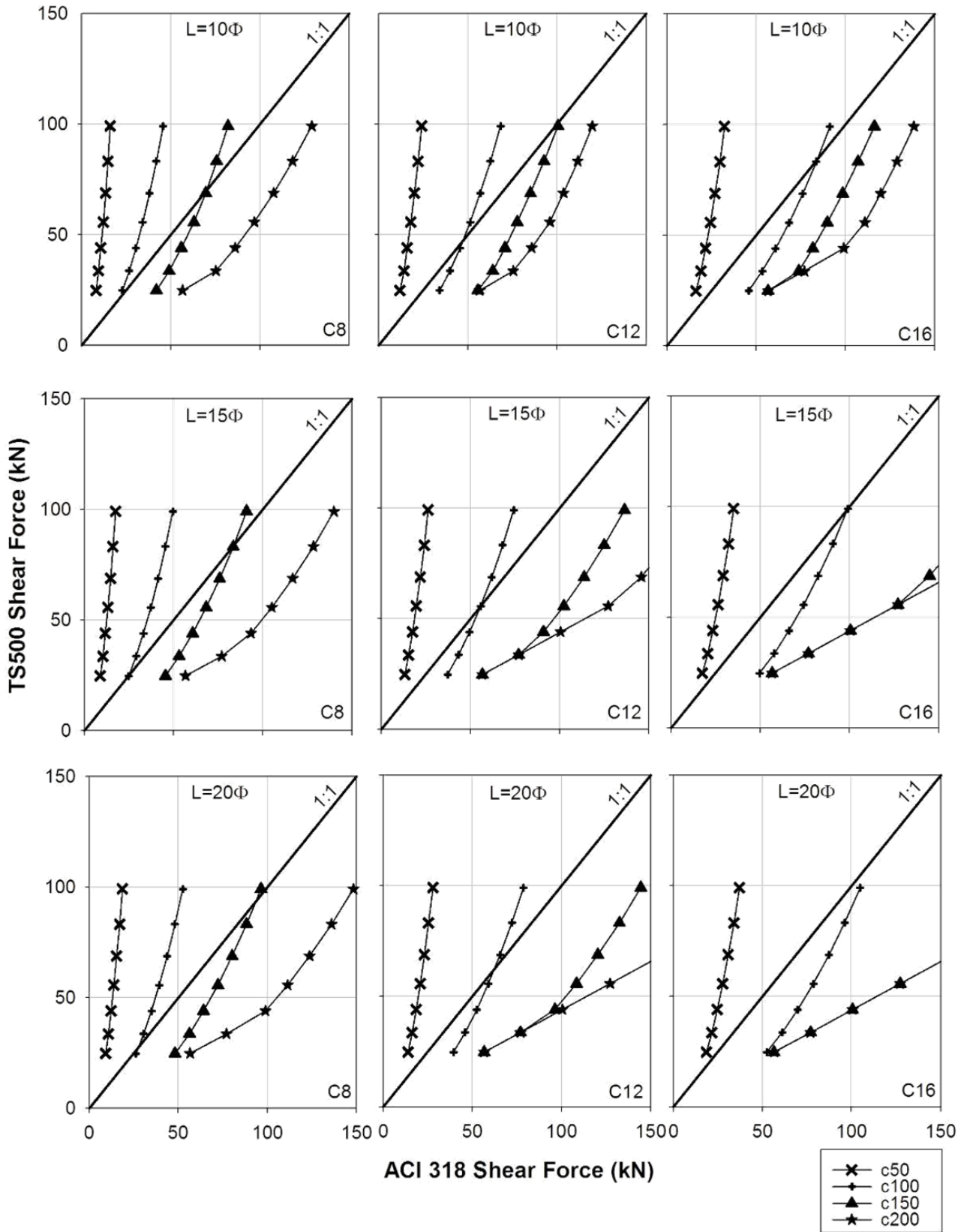
Fig. 3. ACI318 - TS500 comparison of shear forces.
