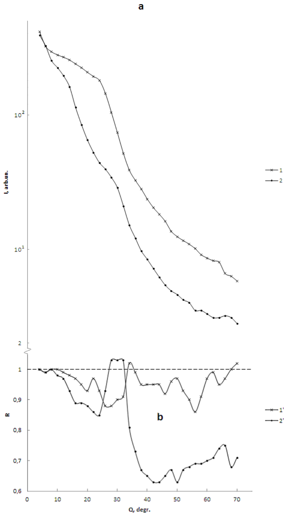
Pic.1.a. Scattering indicatrices of the initial water of the first (curve 1) and second (curve 2) structure degrees.
