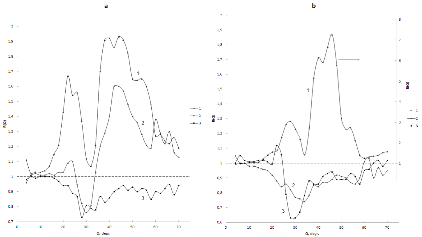
Pic.5. Relative scattering indicatrices of water samples of I degree after the internal mutual influence (a) by informational field and the form field of a pyramid (1), the one of a cylinder(2), the one of a prism (3) for 10 min long and the following exposure for 2 hours long(b) inside the corresponding forms.
