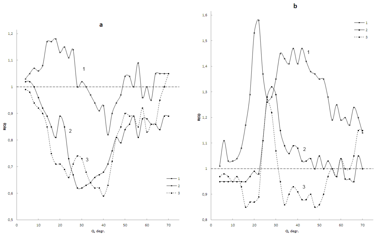
Pic.4. Relative scattering indicatrices of water samples of II degree after the internal (a) and the external (b) influence by the form field of a prism (1), mutual influence by informational and the form fields (2) and the following exposure of water samples inside and outside the form for 1 hour long (3).
