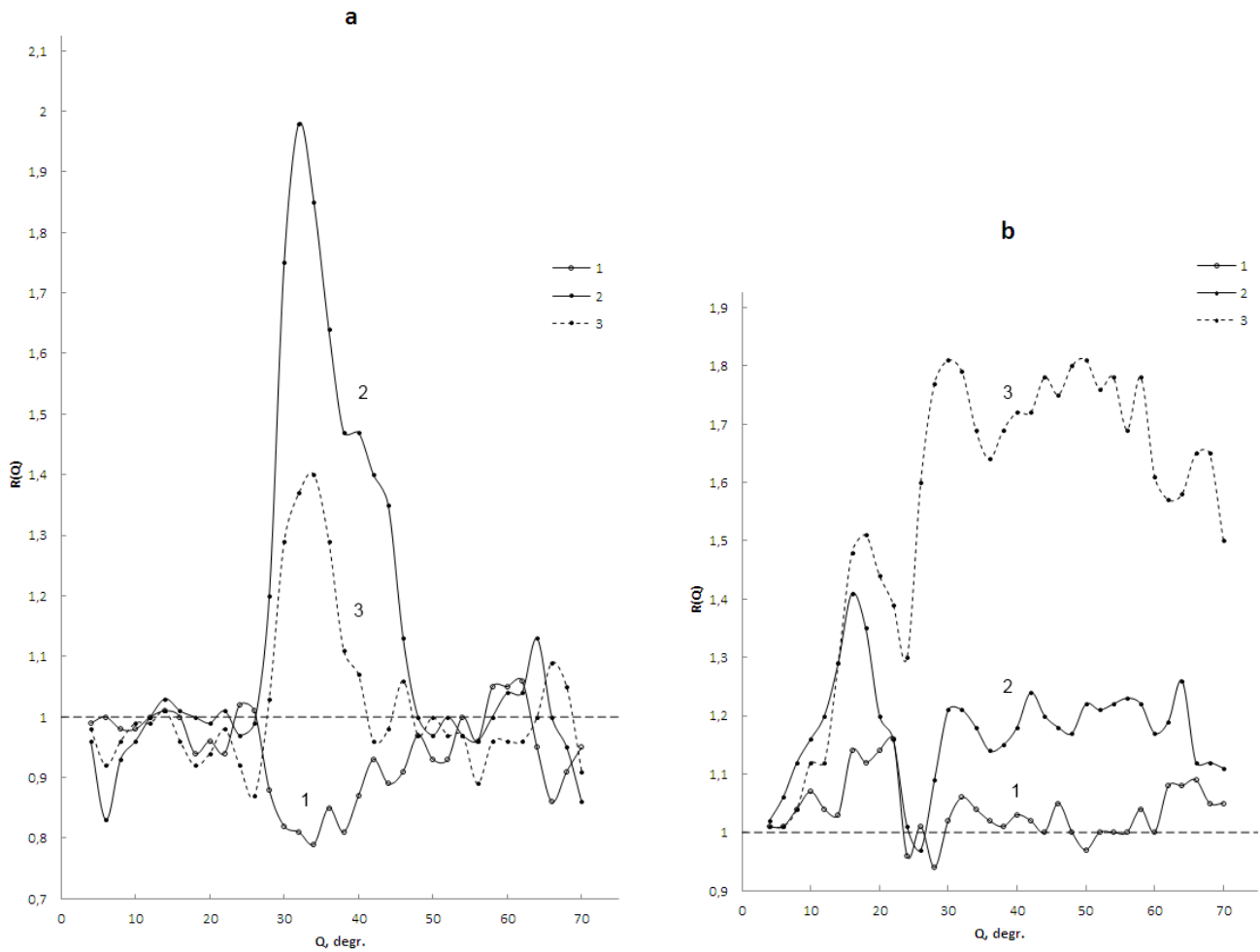
Pic.3. Relative scattering indicatrices of water samples of II degree after the internal (a) and the external (b) influence by the form field of a cylinder (1), mutual influence by informational and the form fields (2) and the following exposure of water samples inside and outside the form for 1 hour long (3).
