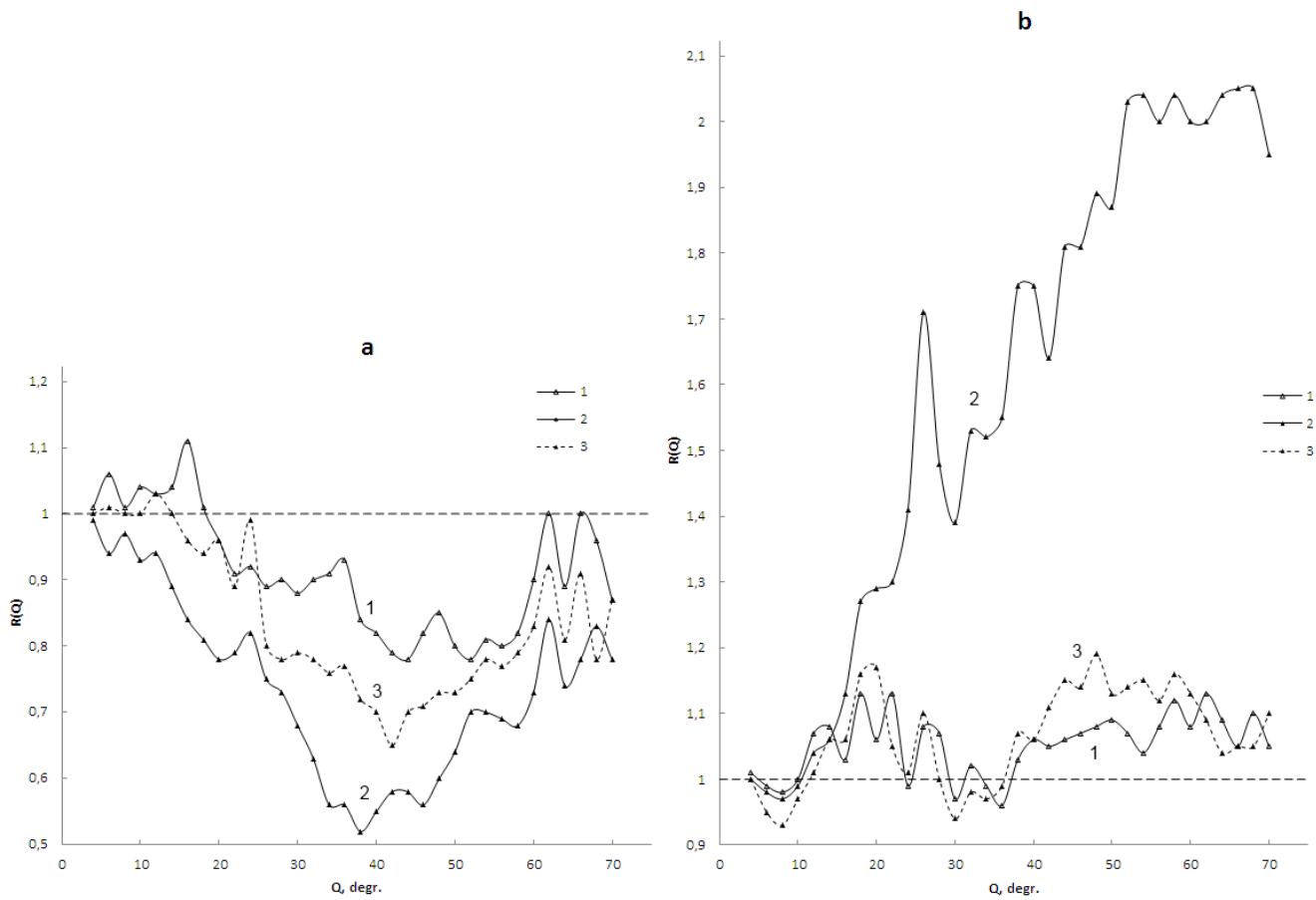
Pic.2. Relative scattering indicatrices of water samples of II degree after the internal (a) and the external (b) influence by the form field of a pyramid (1), mutual influence by informational and the form fields (2) and the following exposure of water samples inside and outside the form for 1 hour long (3).
