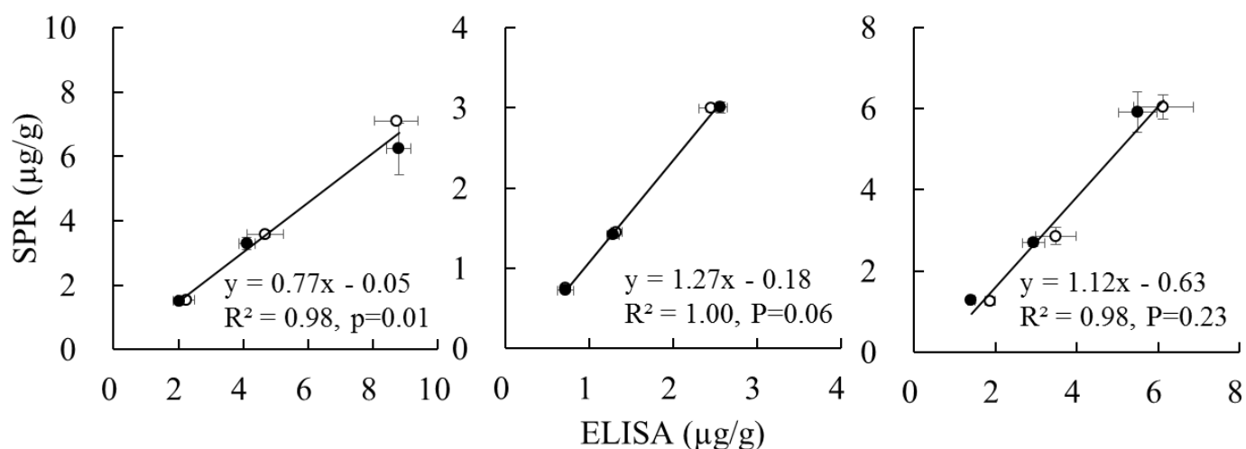
Figure 5. Correlation of pesticide concentrations determined in cucumber ( \circ ) and tomato ( \bullet ) samples spiked with 3 pesticides, between dc-ELISA and SPR-sensor: (A) boscalid hapten immobilized, (B) clothianidin hapten immobilized, (C) nitenpyram hapten immobilized. Each data point is the mean of 3 replicates in independent examinations ; error bars indicate \pm SD.
