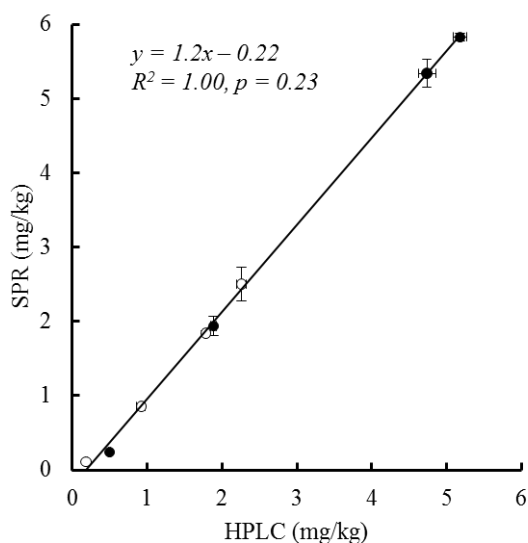
Figure 6. Correlation between the results of the SPR-sensor and the results of HPLC: (○) represents eggplant, and (●) represents cucumber. Each data point is the mean of three replicates from independent examinations. Error bars indicate standard deviations.
