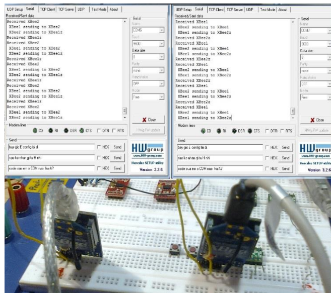
Fig. 10. Communication among XBees
