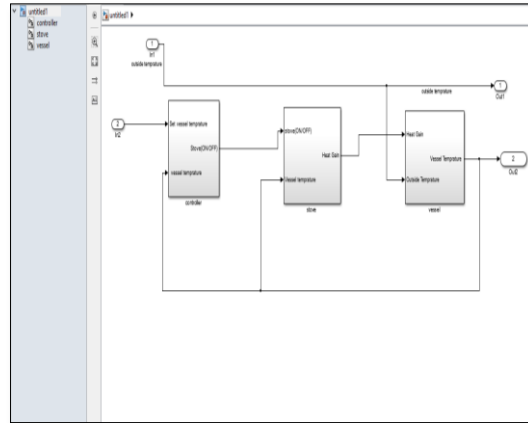
Figure 4. Simulink model to control stove
