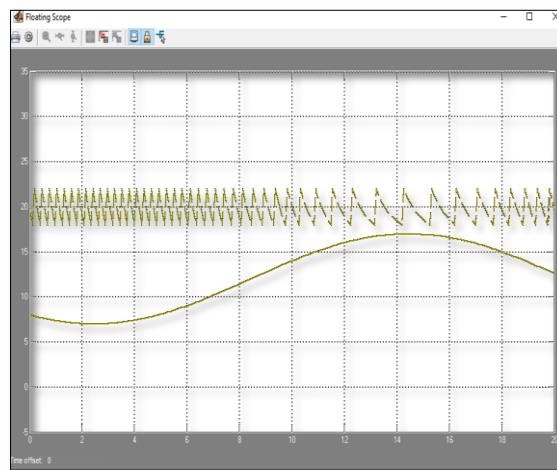
Figure 7. Changing vessel temperature
