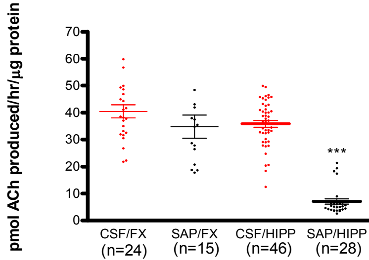
Figure 8: ChAT activity (Corn oil treated rats)
