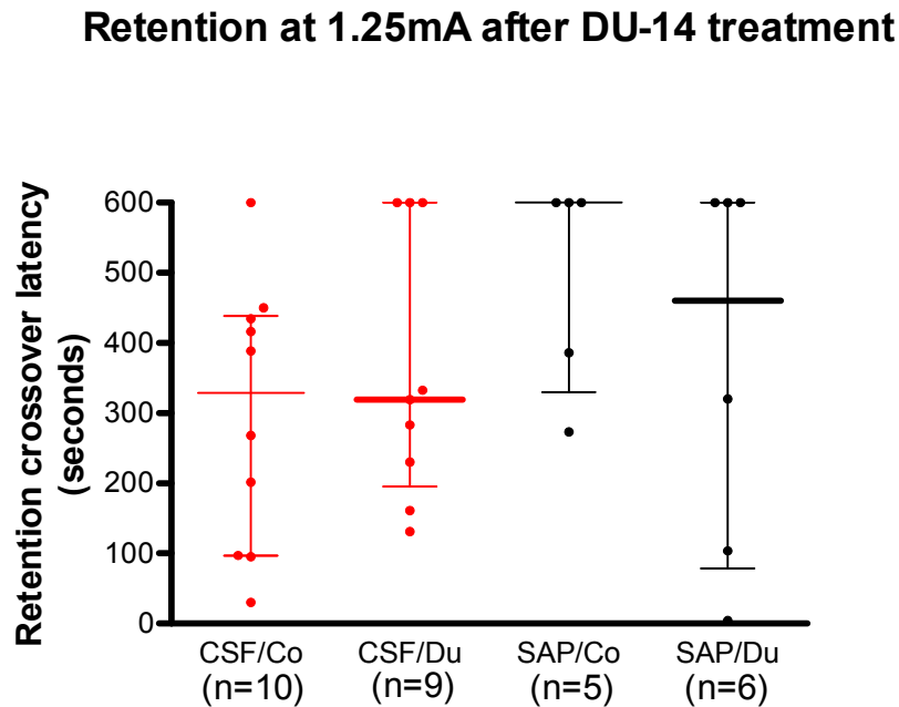
Figure 15: Effect of DU-14 on memory retention after administration of 1.25mA footshock
