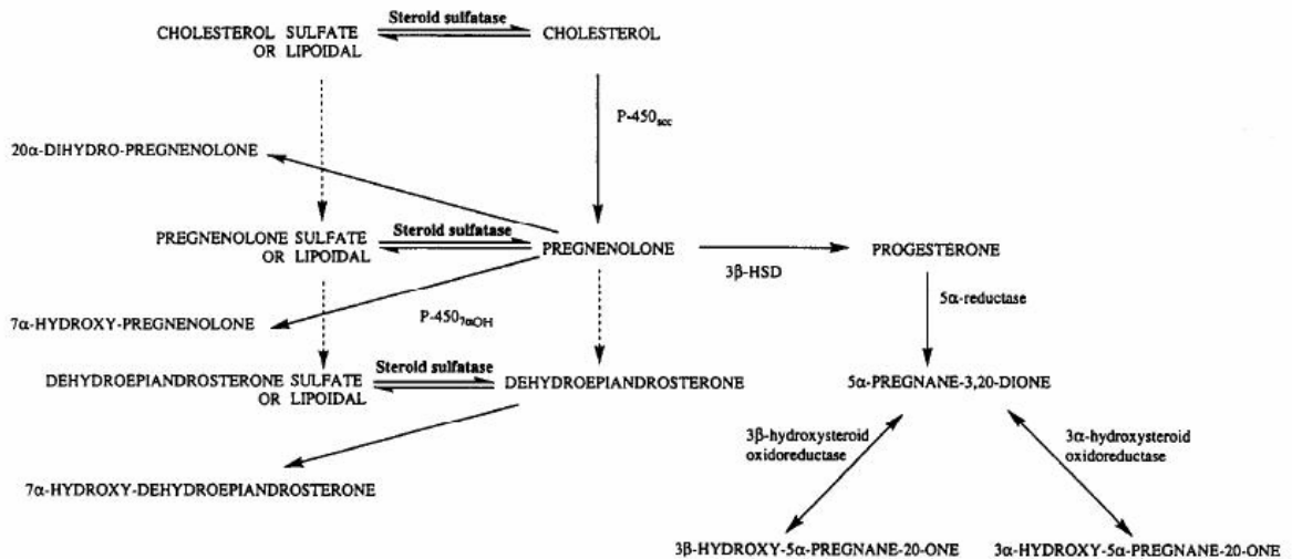
Figure 3: Neurosteroid biosynthesis and metabolism in the rat brain. Dotted arrows indicate metabolic conversions not yet formally demonstrated [5].
