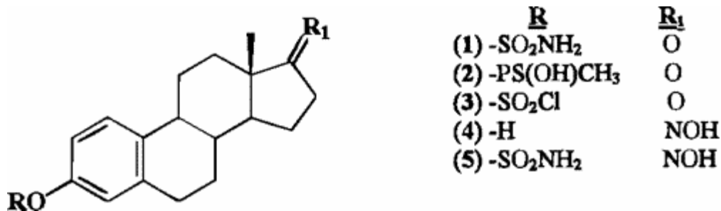
Figure 4: Structures of steroid sulfatase inhibitors (1-3, 5) and estrone oxime (4)
