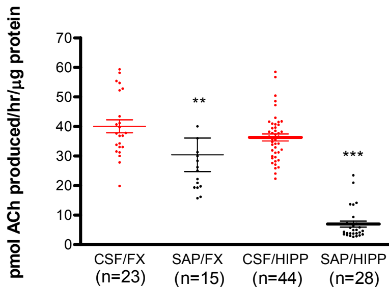
Figure 12: Effect of 192 SAP infusions on ChAT activity in frontal cortex and hippocampal tissues (DU-14 rats)
