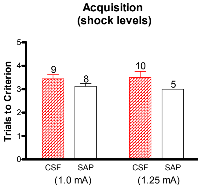
Figure 10: Effect of shock intensity on memory acquisition
