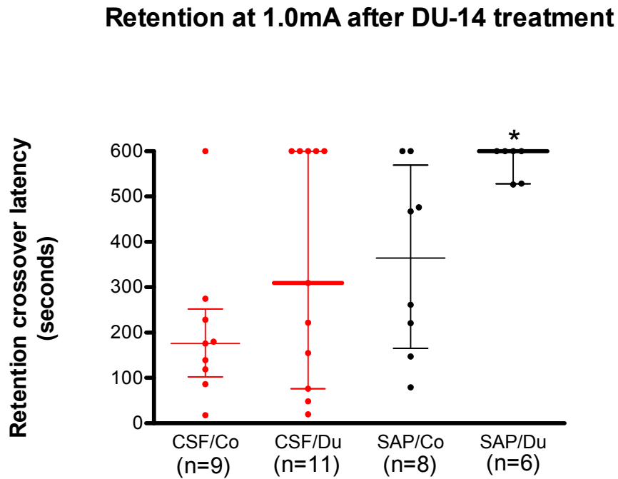
Figure 14: Effect of DU-14 on memory retention after administration of 1.0mA footshock
