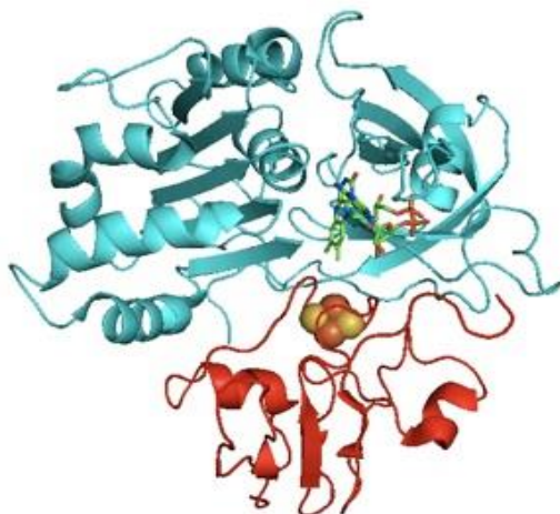
Figure 1: The crystal structure of the Fdx-FNR complex in the early stages of association during electron transfer. The top (blue) depicts the FNR, whereas the bottom (red) depicts the Fdx 14 .
