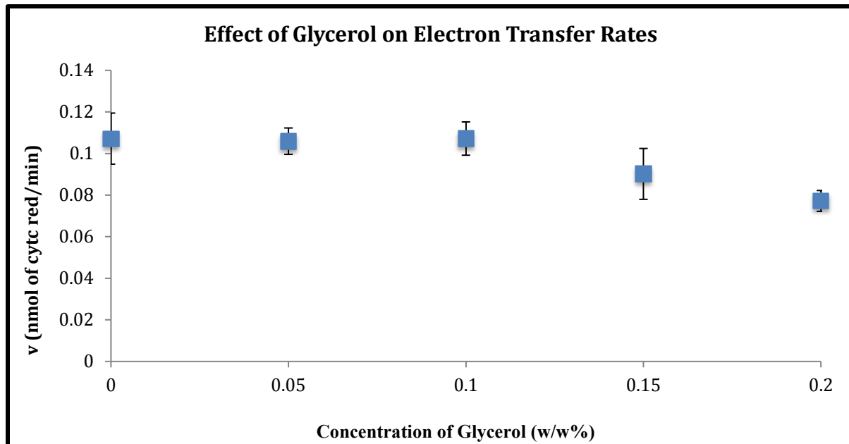
Figure 3: Effects of glycerol on kinetics of cytochrome c reduction. Error bars represent a standard deviation.
