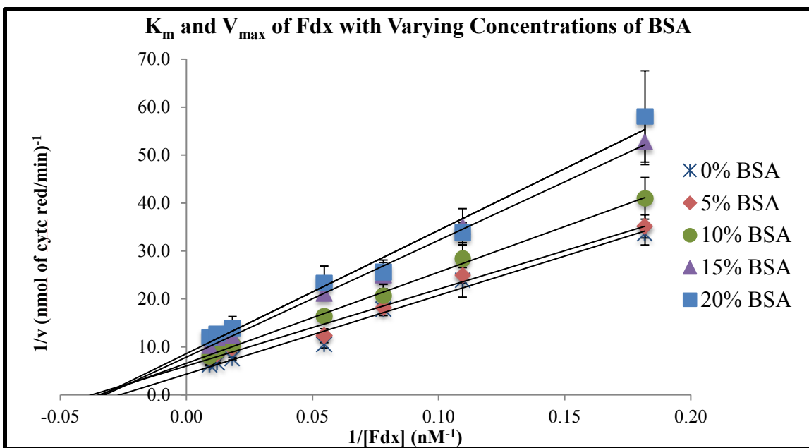
Figure 2: Effects of bovine serum albumin (BSA). Double reciprocal plots show a comparison of kinetic assays in the presence of 0%, 5%, 10%, 15%, and 20% BSA. Error bars represent a standard deviation.
