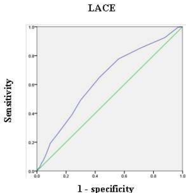
Figure 1. Determine the cut-off point in the index LACE with use receiver operating characteristic curve
