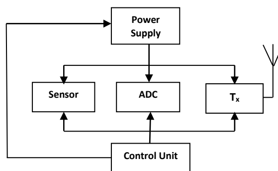
Fig. 1. Basic Architecture of proposed wireless sensor node.
