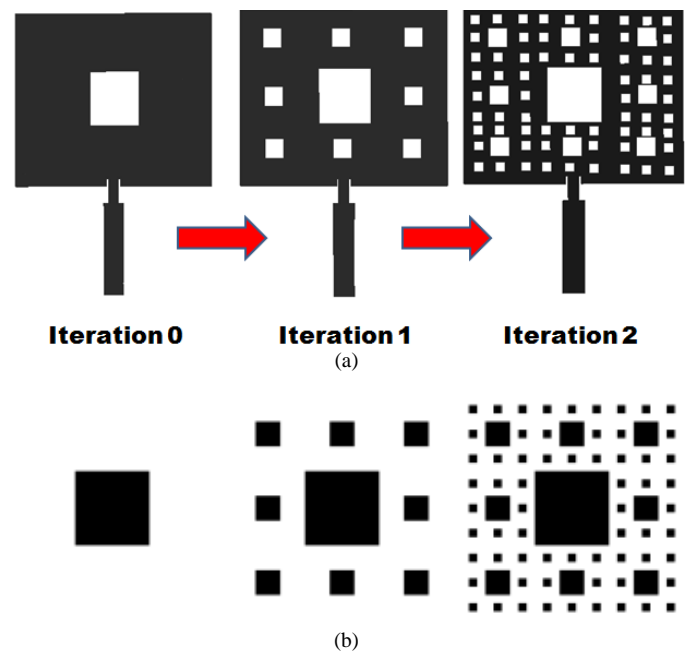
Fig. 2. Design Evolution
