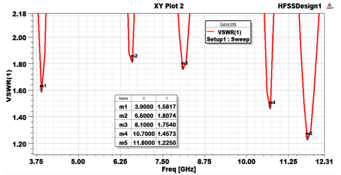
Fig. 5. VSWR plot of the proposed antenna
