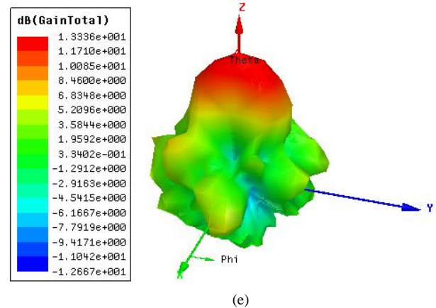
Fig. 8. Simulated Gain at (a) 3.9, (b)6.6, (c) 8.1, (d) 10.7, & (e) 11.8 GHz
