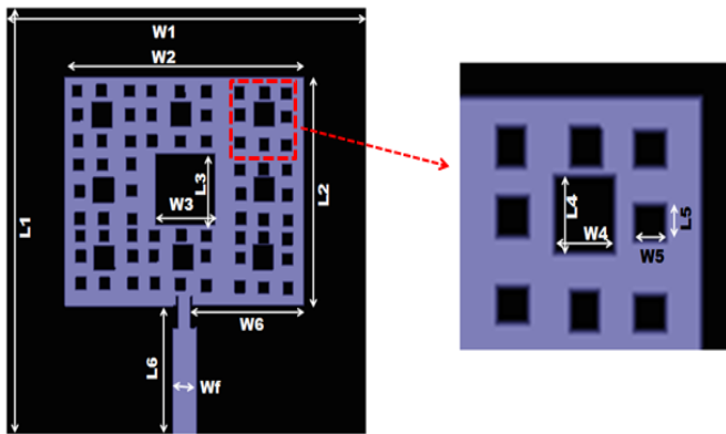
Fig. 1. Physical layout of the proposed antenna
