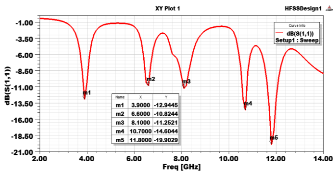
Fig. 4. Simulated S_{11} (reflection coefficient) of the proposed design
