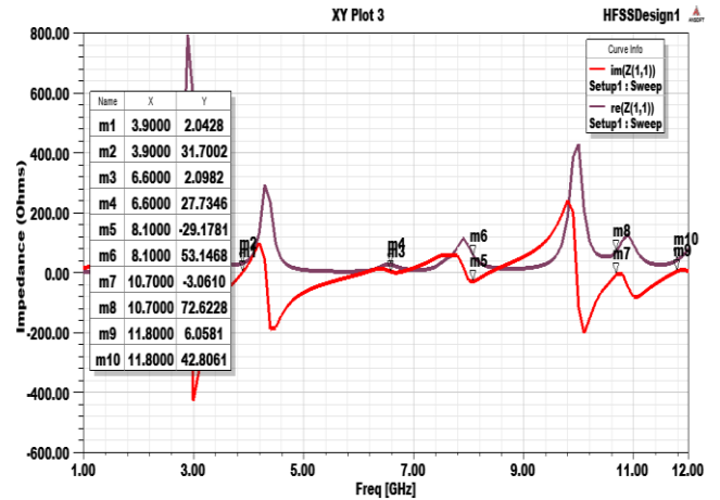
Fig. 6. Simulated input impedance
