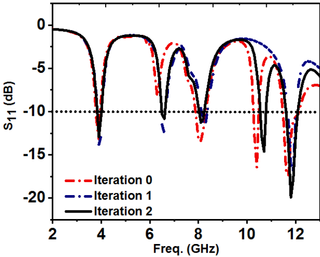
Fig. 3. S_{11} Evolution plot of the proposed antenna
