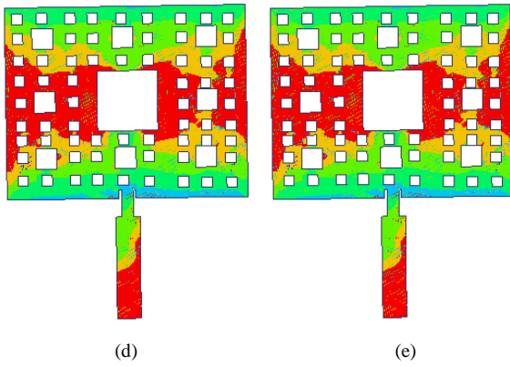
Fig. 7. Distribution of surface Current at (a) 3.9, (b)6.6, (c) 8.1, (d) 10.7, and (e)11.8 GHz
