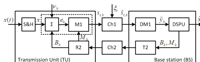
Fig. 1. Block diagram of optimal AFCS.
