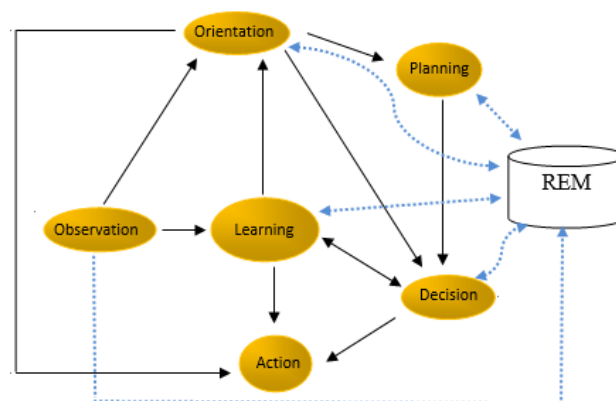
Fig. 1. REM role in the cognitive cycle [4]
