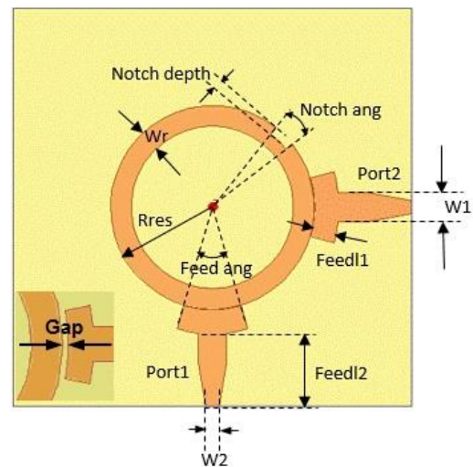
Fig. 2. Initially designed filter. .Dimensions are in (mm): R_{res} = 15.3 , Gap = 0.2, Feed1 = 2.4, Feed2 = 11.8, w_1 = 3.5 , w_r = 3.21 , w_2 = 2 , Notch-depth = 1.28, Notch-ang = 12^\circ , Feed ang = 40^\circ
