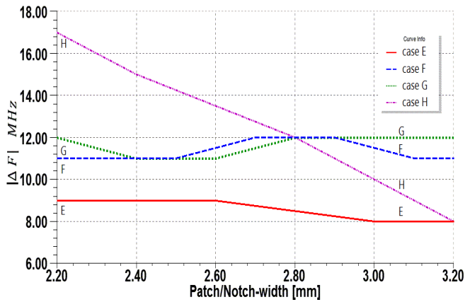
Fig. 10. Dual mode circular ring BPFs, perturbed by different cases of rectangular perturbation elements at azimuthal angles of 45°
