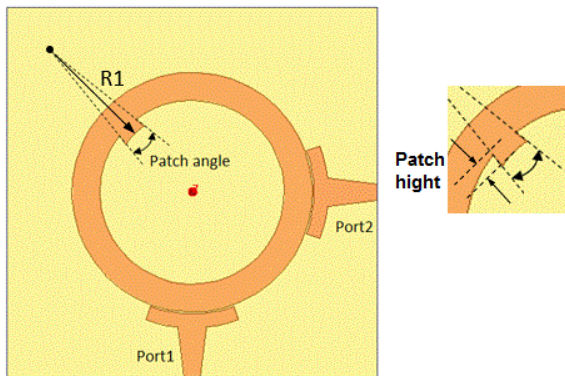
Fig. 11. Dual mode circular ring BPFs, perturbed by inner radial patch at azimuthal angle of 135°. Main Dimensions are in (mm): R_{res} = 15.33 , R1 = 14.65 , wr = 3.33 , Notch-height = 1.28
