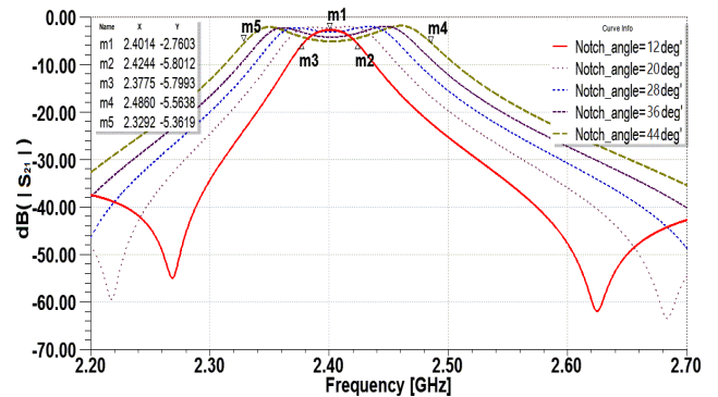
Fig. 6. Frequency responses ( |S_{21}| ) of the filter for several notch-angle values at notch notch- depth to 1.2 mm
