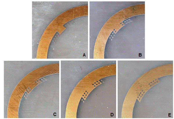
Fig. 15. Fabricated samples for the five cases of the perturbation element
