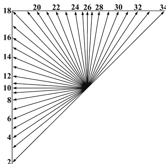
Fig. 1. HEVC angular intraframe prediction modes.
