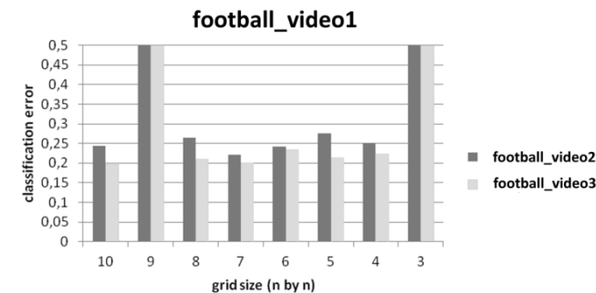
Fig. 19. The results for the Artificial Neural Network.
