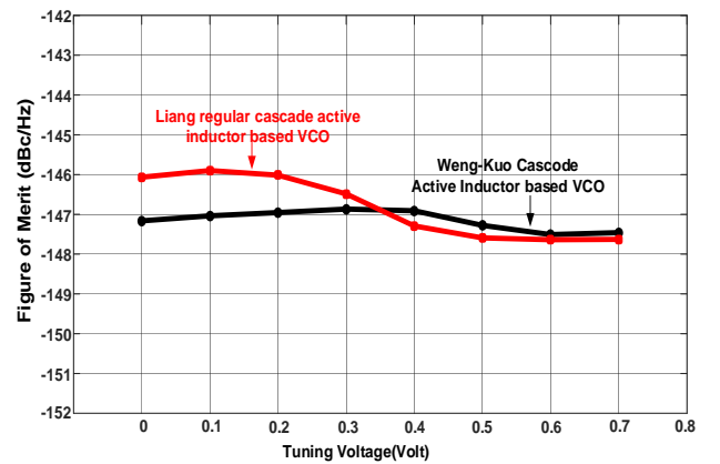
Fig. 12. Figure of merit vs tuning voltage for the proposed VCOs.
