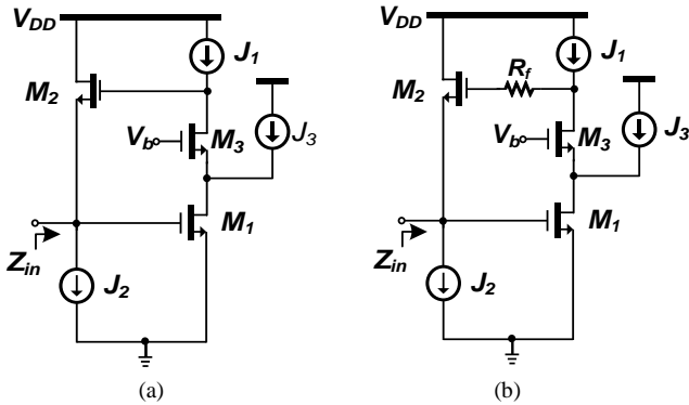
Fig. 2. Weng- Kuo Cascode active inductor. (a) Without feedback resistor. (b) With feedback resistor.
