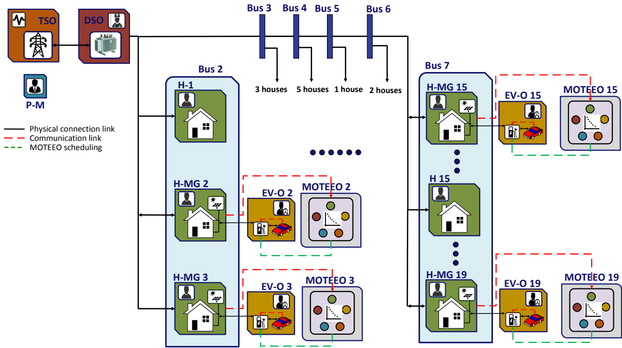
Figure 2 MOTEEEO framework for a distribution network
