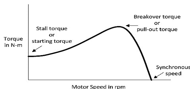
Fig. 1: Torque Vs motor Speed diagram.
