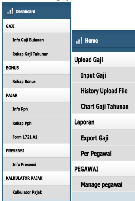
Gambar 5 Menu Samping
