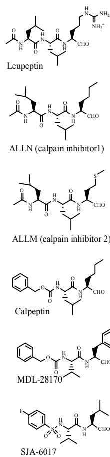
Figure 7. Typical calpain inhibitors.
