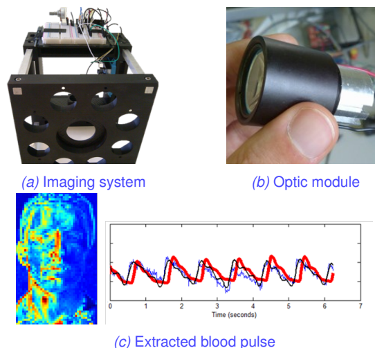
Fig. 1: Imaging system overview. The chassis (a) incorporates a solid base designed for mounting a scientific camera and electronics, and a length-adjustable front with eight slots for custom optics (b). This system can be used, for example, to extract blood pulse fluctuations across a spatial area (c).
