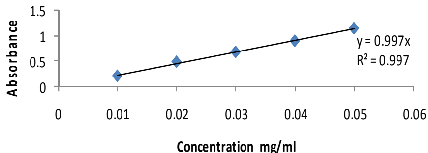
Figure 1: Beer-Lambert's plot for pure metformin
