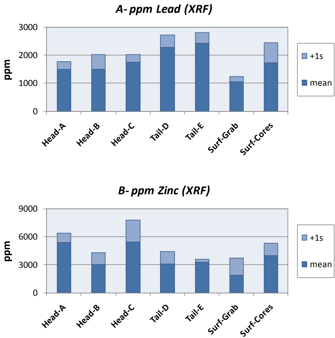
Figure 18: Metal Contaminant Variability Among in Bar Cores and Surface Samples
