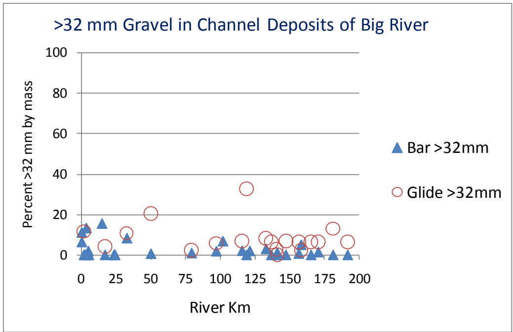
Figure 14: Coarse Gravel Distribution in Bar and Glide Samples
