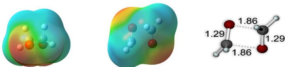
Figure 30. 1,3-dioxetane [2+2] SS B3LYP/6-31G(d) TSS. Electrostatic potential map and stationary point geometry. Isovalue -4.00e-2 to 4.00e-2 . Distances in angstroms.
