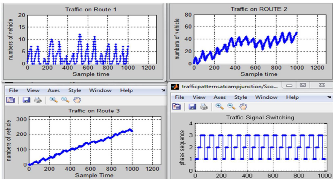
Figure 12: The result for the fixed time controller
