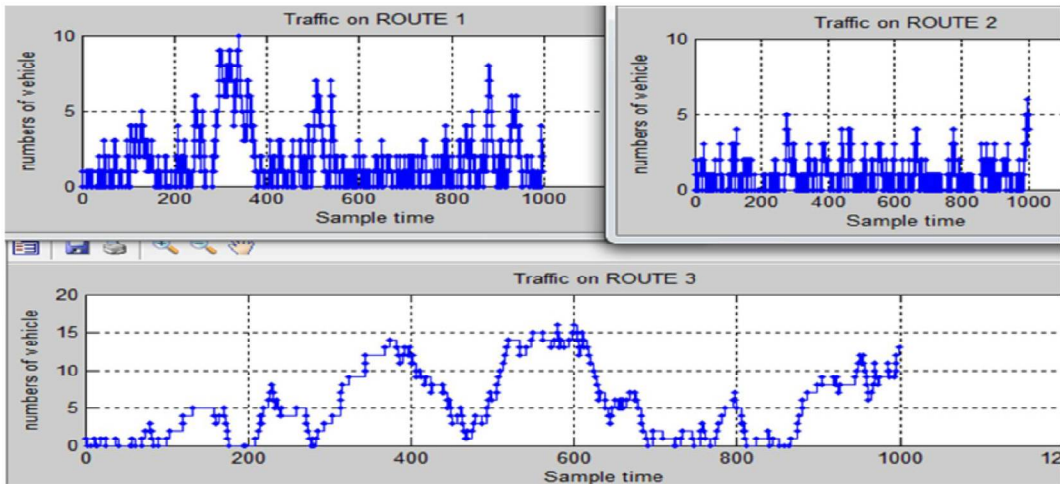
Figure 11: Results for the fuzzy controller
