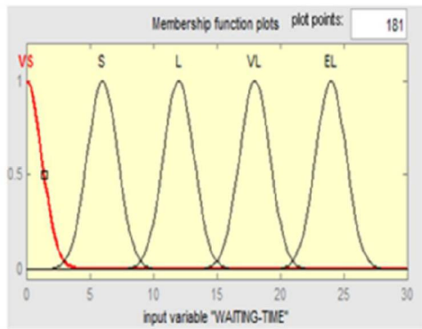
Figure 8: Input membership functions of vehicles queue
