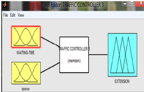
Figure 6: Fuzzy traffic control unit
