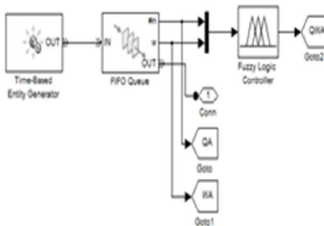
Figure 10: FLC subsystem model of each approach
