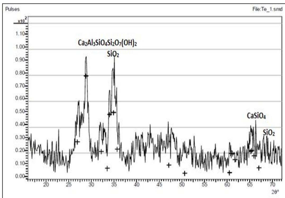
Plate 5: XRD spectrum for Wood ash
