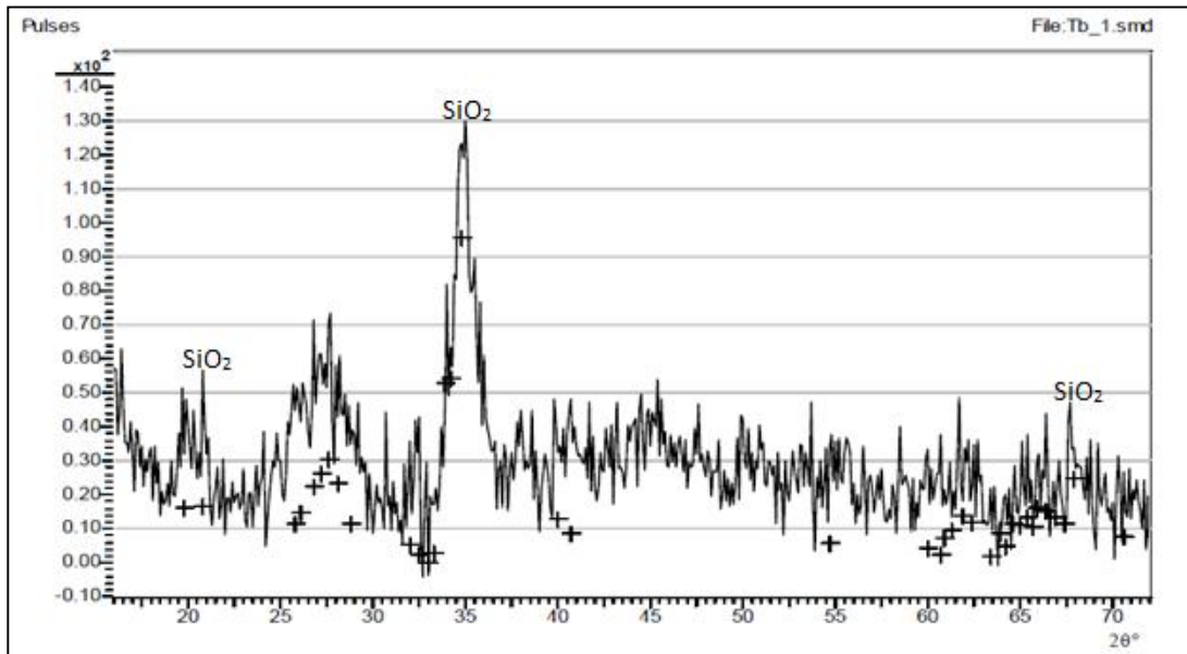
Plate 2: XRD spectrum of Quartzitic clay
