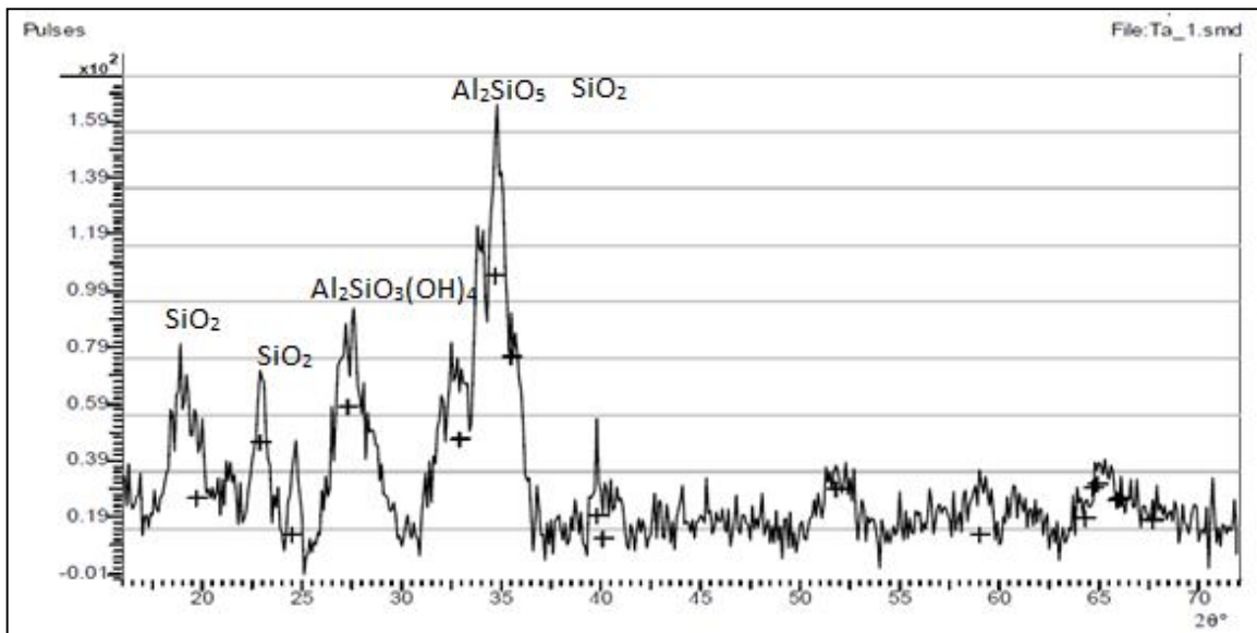
Plate 1: XRD spectrum for Kaolinitic clay.
