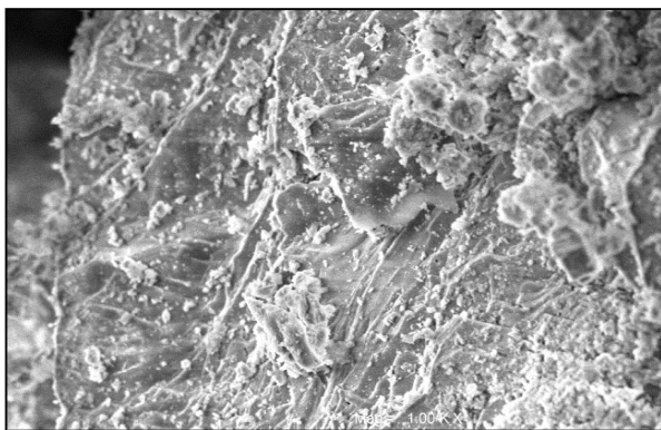
Plate 6: SEM of procelainised stoneware tile without wood ash M x 5000
