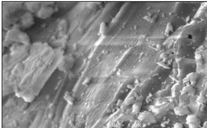
Plate 9: SEM of porcelainised stoneware tile with (kaolinitic clay) 5% wood ash M X 5000
