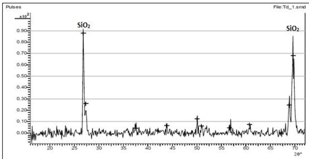
Plate 4: XRD spectrum for Quartz
