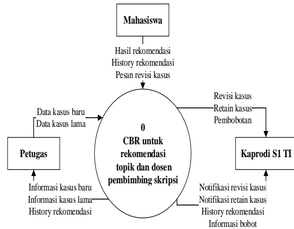
Gambar 5. DFD Level 0
