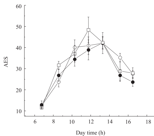
Figure 3. Daily course of alternative electron sink (AES) in bean genotypes 'Carioca' (○), 'Guarumbé' (●) and 'Ouro Negro' (□) exposed to daily changes of environmental variables in Piracicaba, SP, Brazil. Each point represents the mean \pm standard error of six replications.
