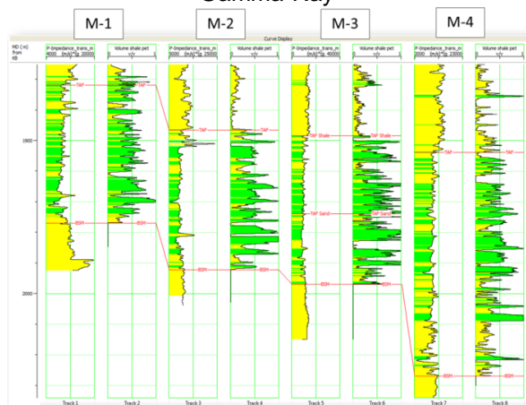
Gambar 17. Cross-section hasil analisis sensitivitas P-Impedance vs V-shale
